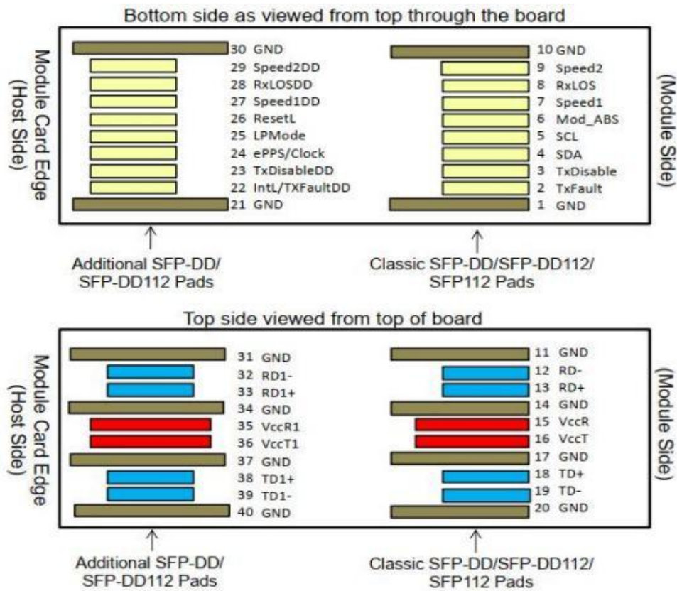
Figure 2. Electrical Pin-out Details
