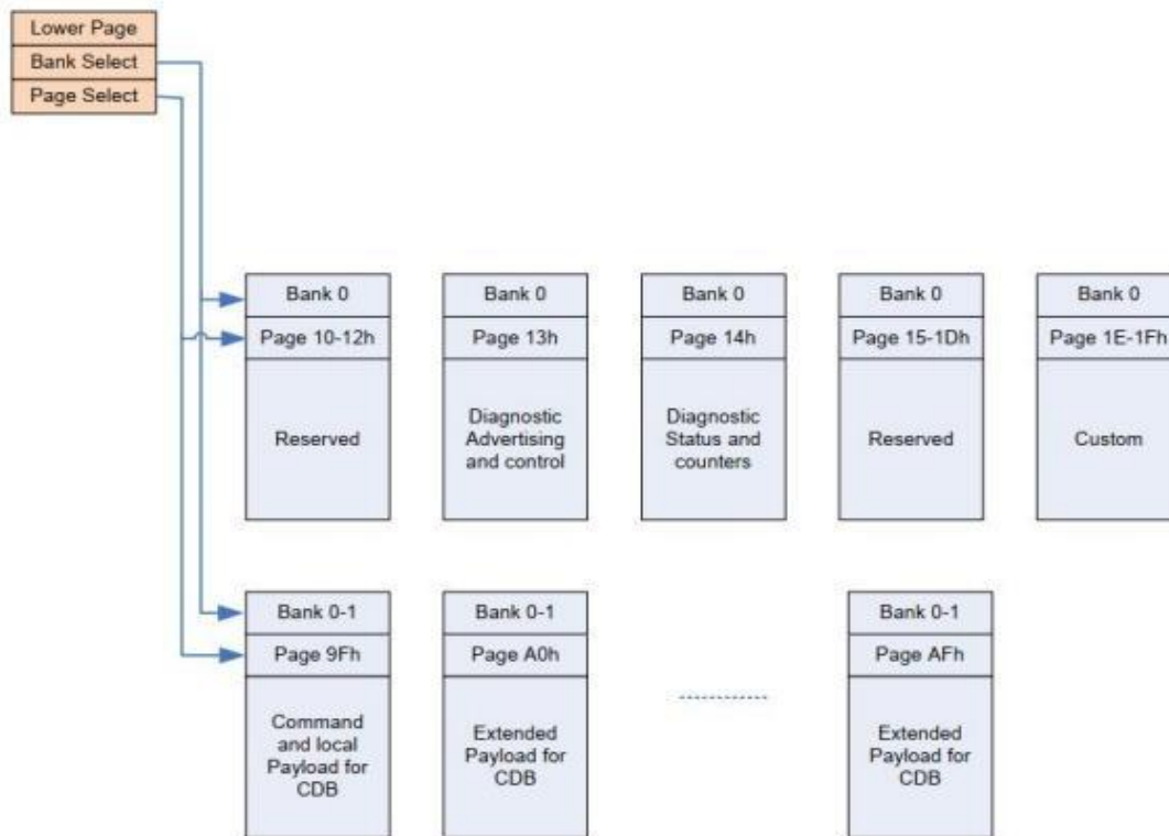
Figure 5. SFP-DD MIS Bank Page Memory Map
