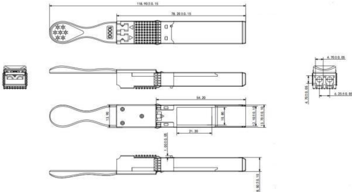
Figure 11. Mechanical Specifications
