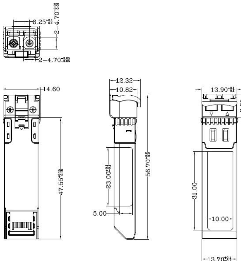
Figure 6. Mechanical Drawing
