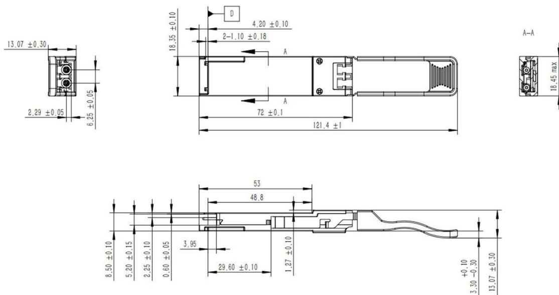
Figure 2. Mechanical dimensions
