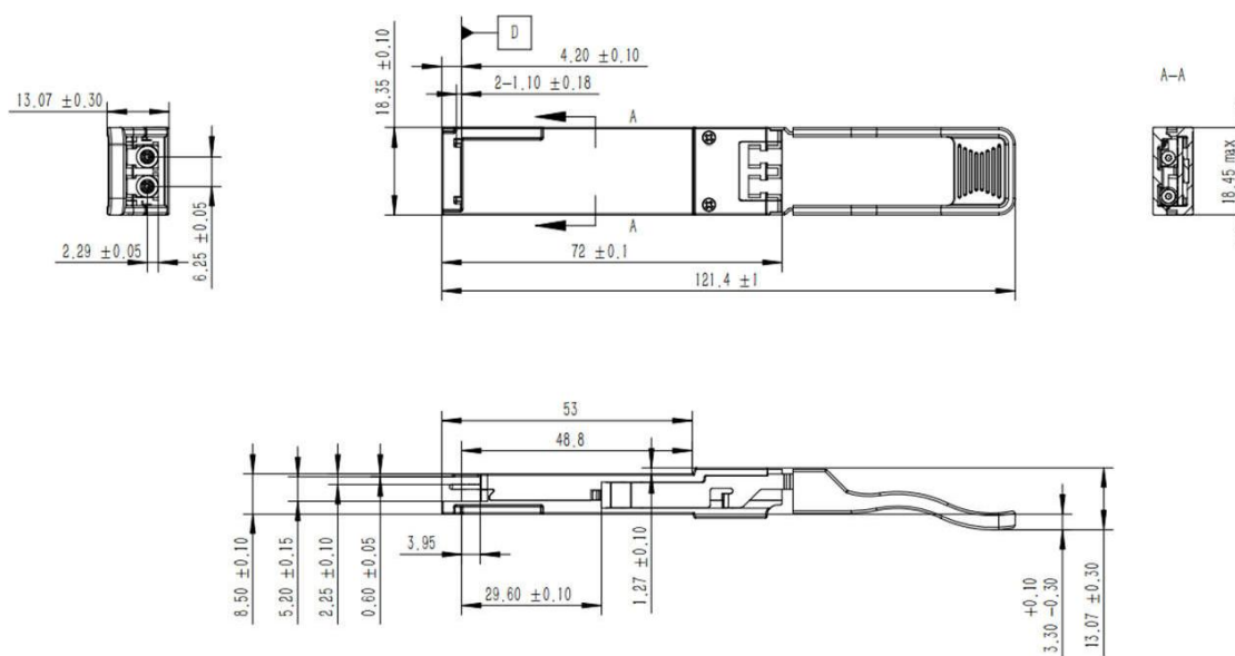
Figure 2. Mechanical dimensions
