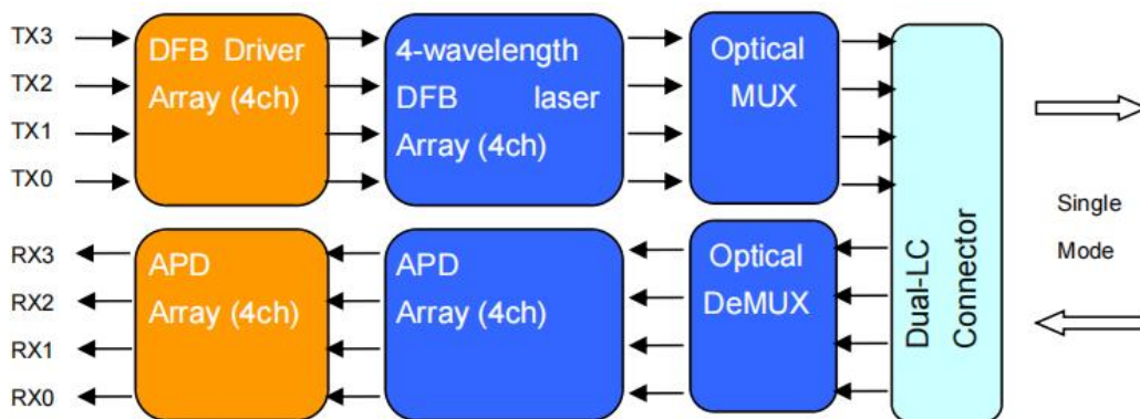
Figure 1: 40Gb/s QSFP ZR4 Transceiver Block Diagram
