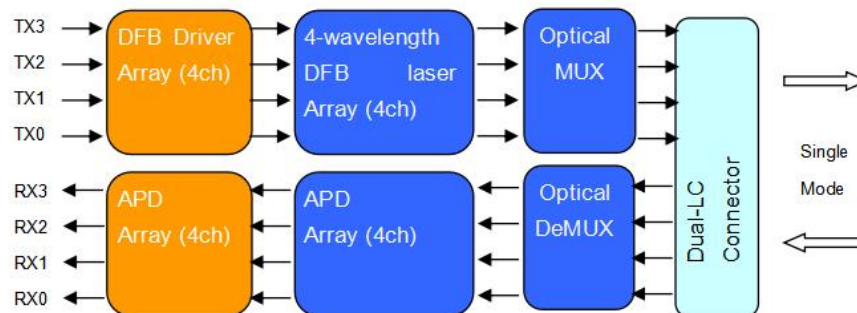
Figure 1: 40Gb/s QSFP ER4 Transceiver Block Diagram
