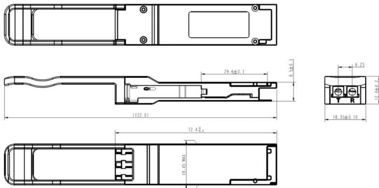
Figure 3. Mechanical Dimensions
