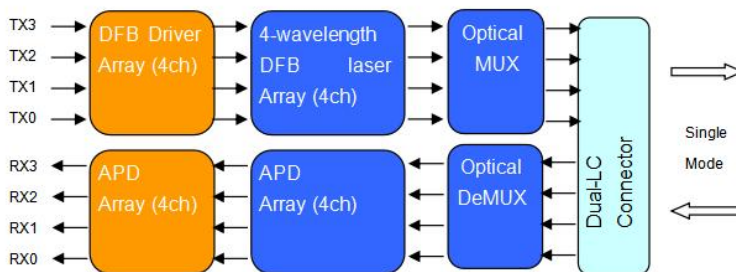
Figure 1: 40Gb/s QSFP ER4 Transceiver Block Diagram
