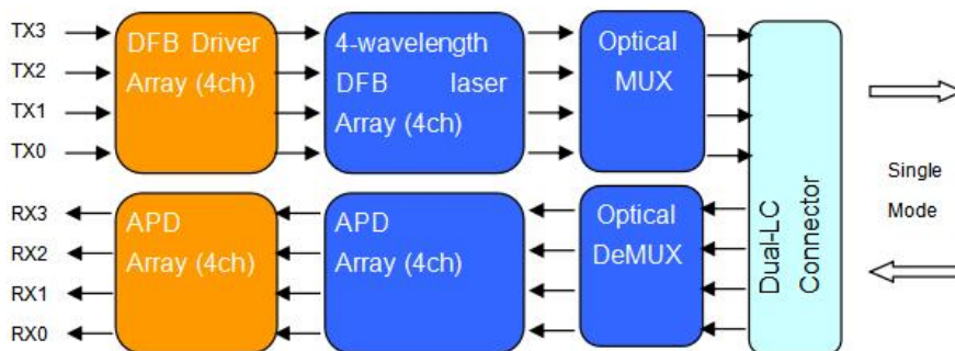
Figure 1: 40Gb/s QSFP ER4 Transceiver Block Diagram
