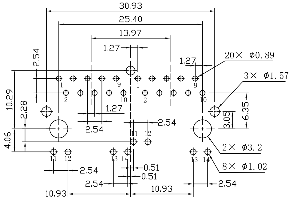
SUGGESTED PCB LAYOUT (TOP VIEW)
