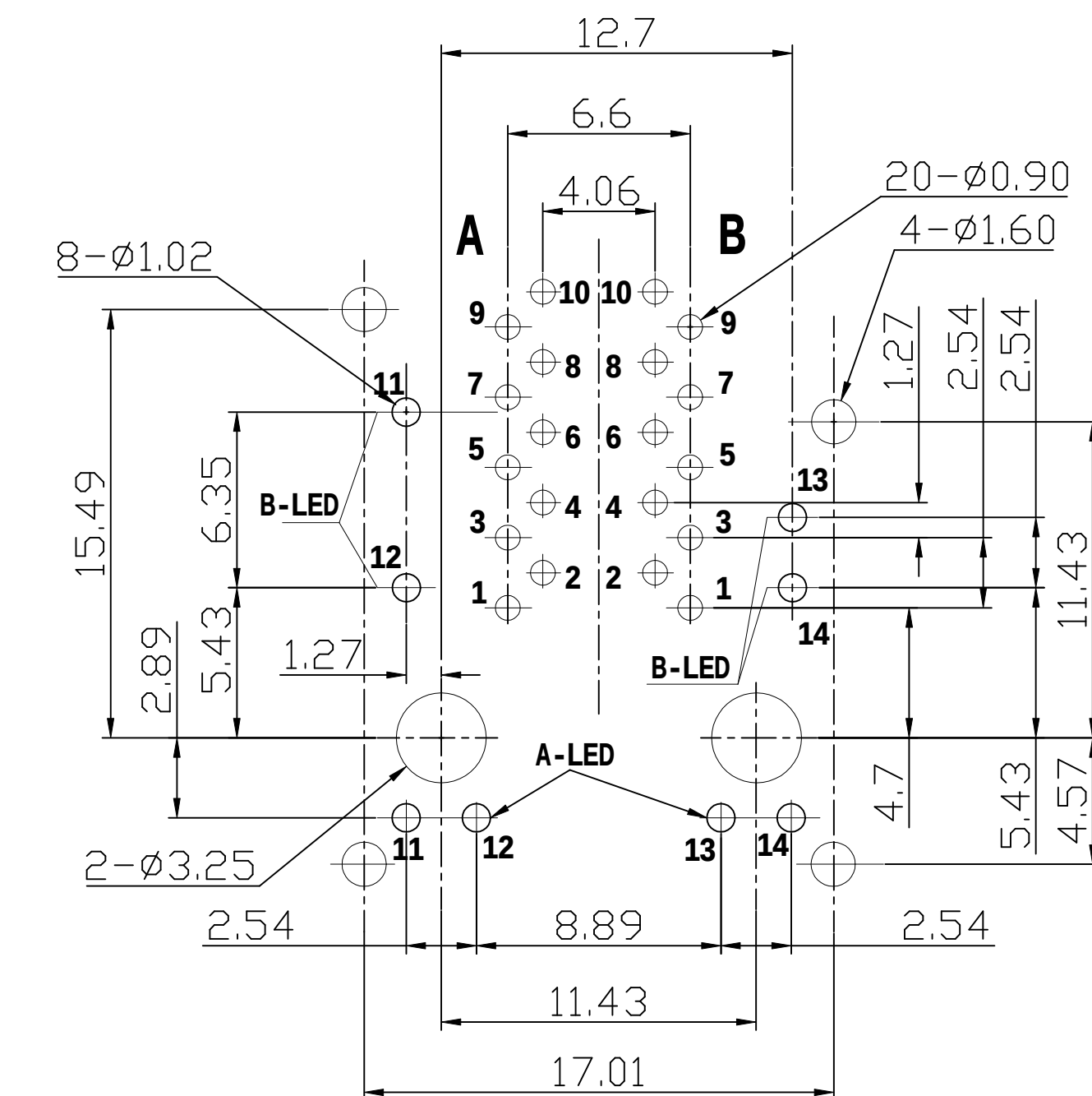
RECOMMENDED PCB LAYOUT(TOP VIEW)
