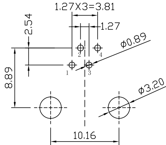
PC Board Layout (Top View)
