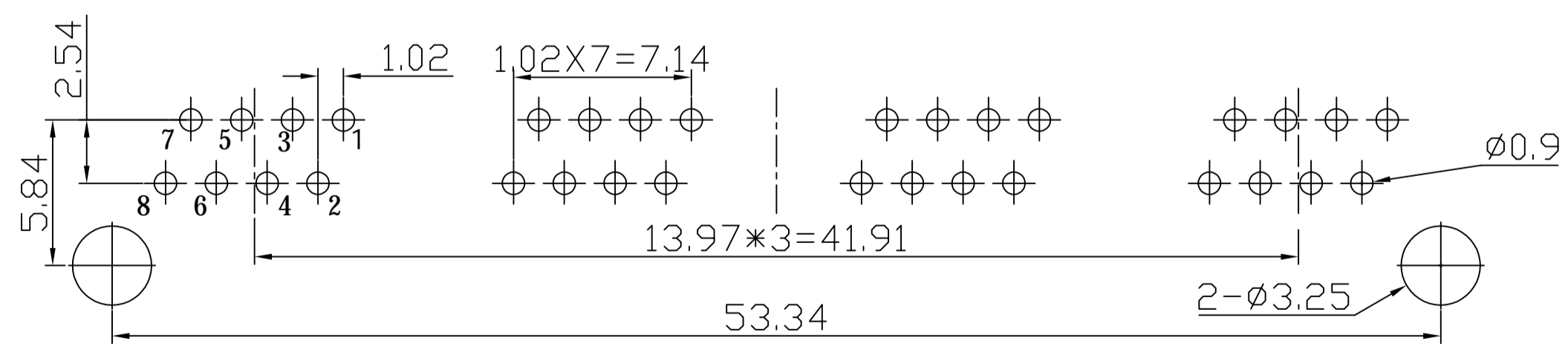
RECOMMENDED PCB LAYOUT(TOP VIEW)
