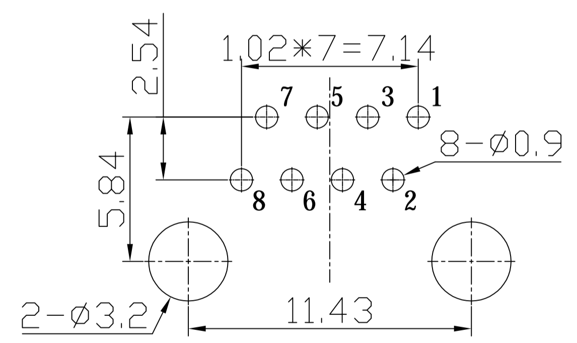
RECOMMENDED PCB LAYOUT(TOP VIEW)
