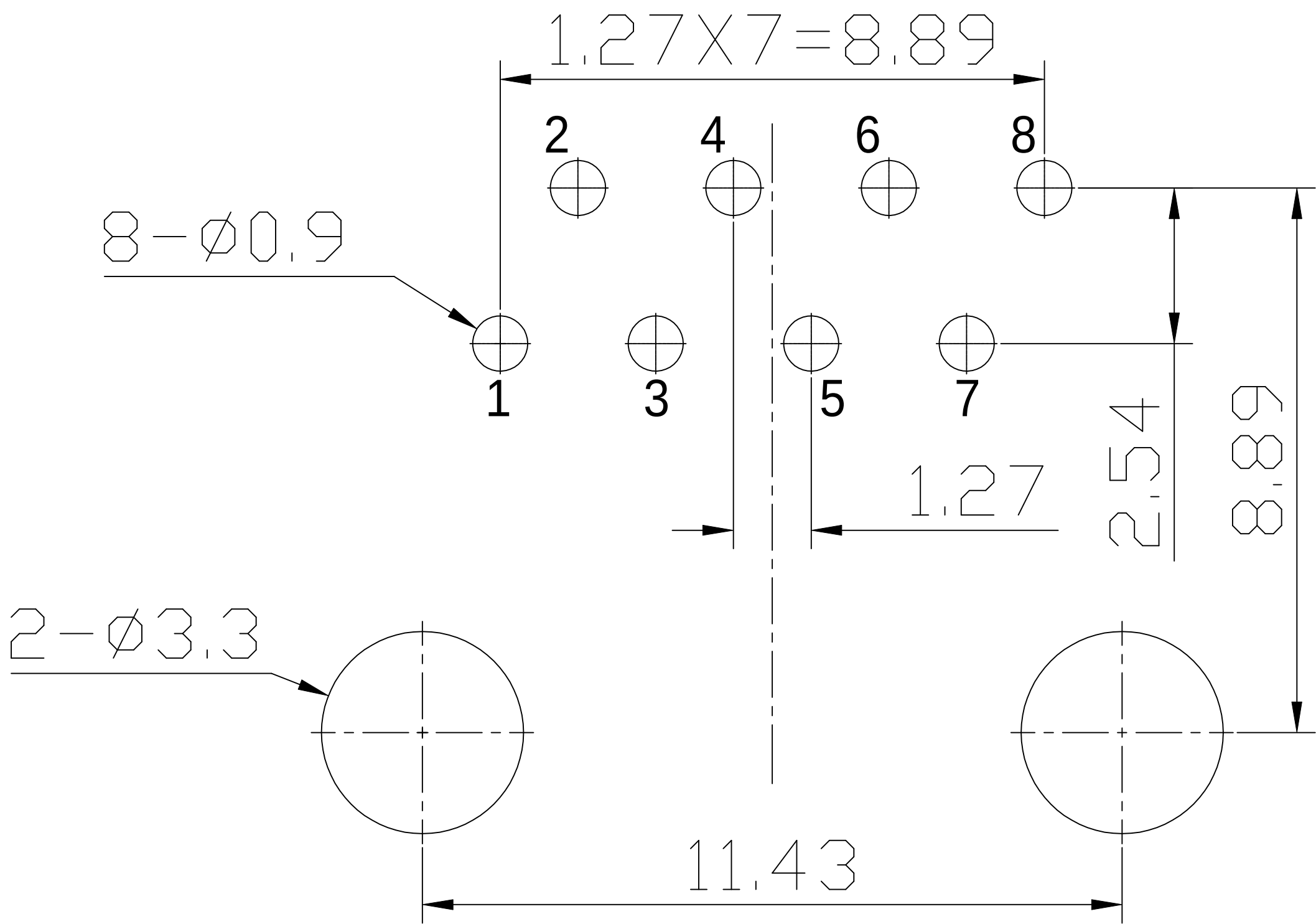
RECOMMENDED PCB LAYOUT(TOP VIEW)
