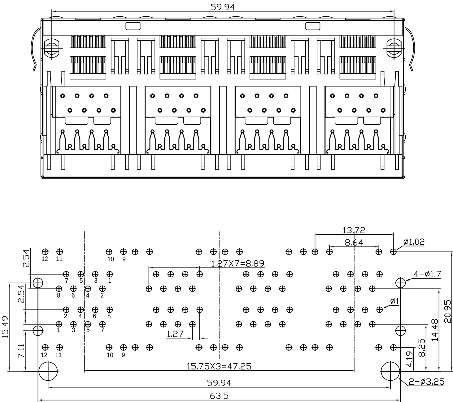
RECOMMENDED PCB LAYOUT(TOP VIEW)
