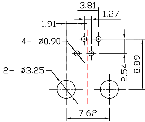
PC Board Layout (Top View)
