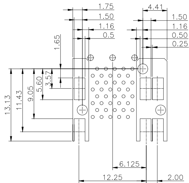
DETAIL-KEEPOUT ZONES
