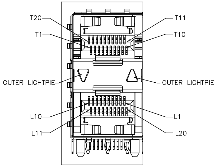
DETAIL A CIRCUIT NUMBERING AND LIGHTPIE INDENTIRICATION
