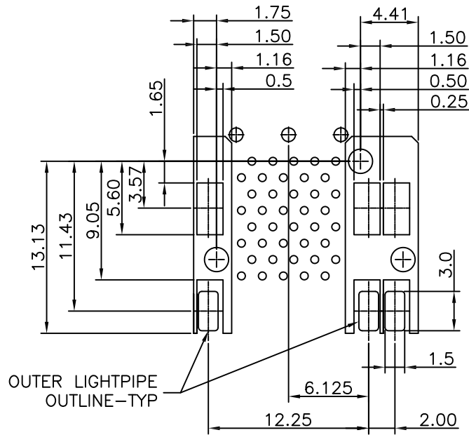
DETAIL-KEEPOUT ZONES
