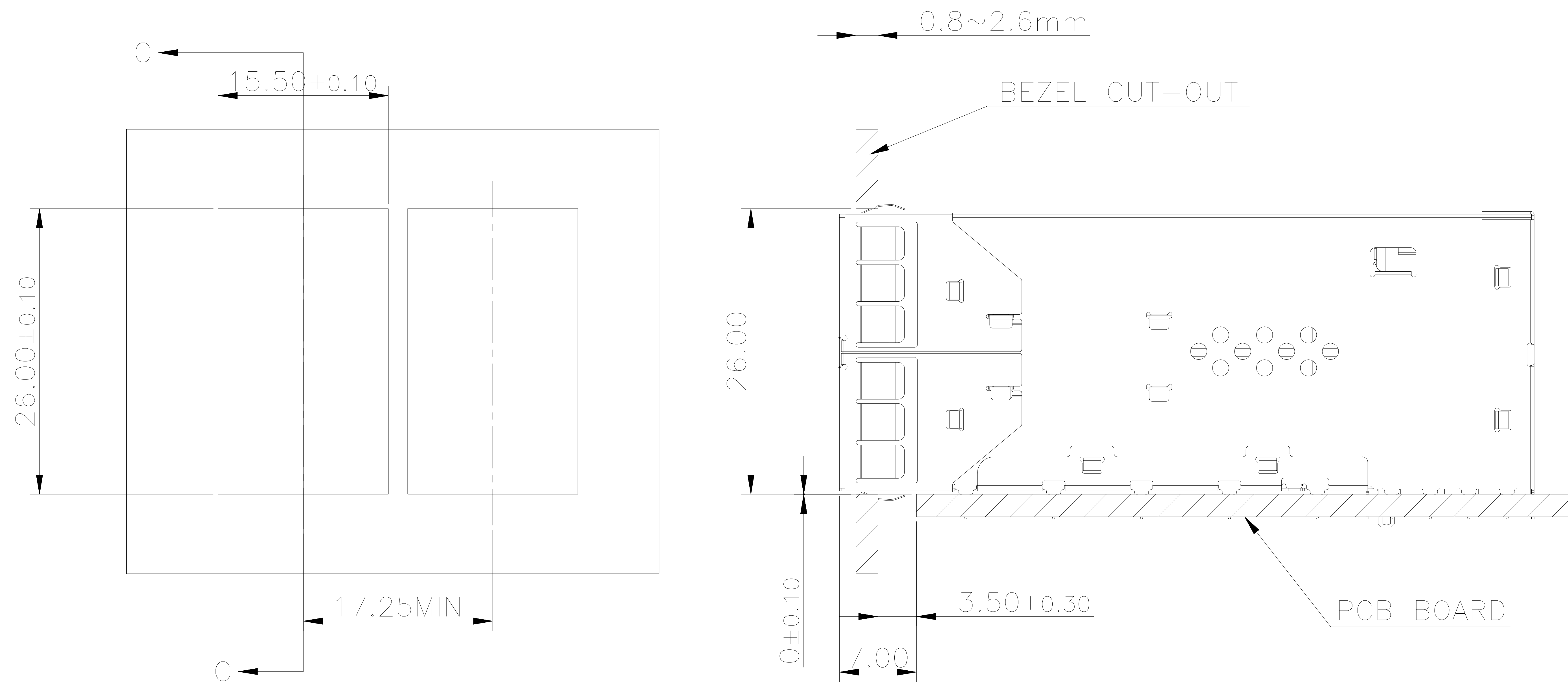
BEZEL CUT-OUT CENTER SPACING DETAIL BEZEL THICKNESS:0.8-2.6
