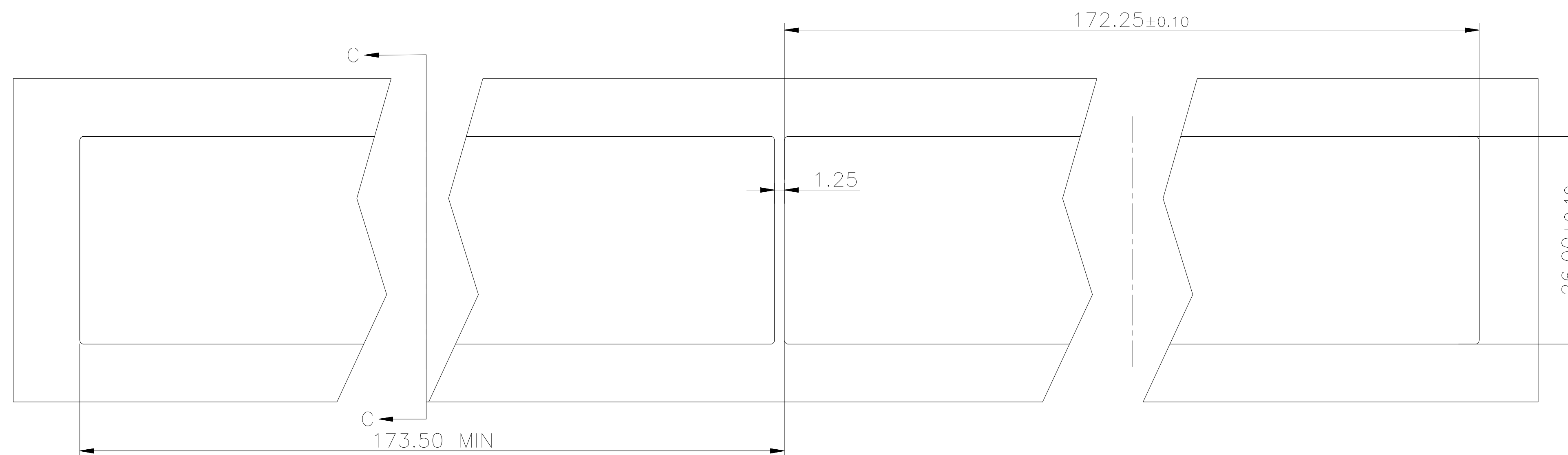
BEZEL CUT-OUT CENTER SPACING DETAIL BEZEL THICKNESS:0.8-2.6
