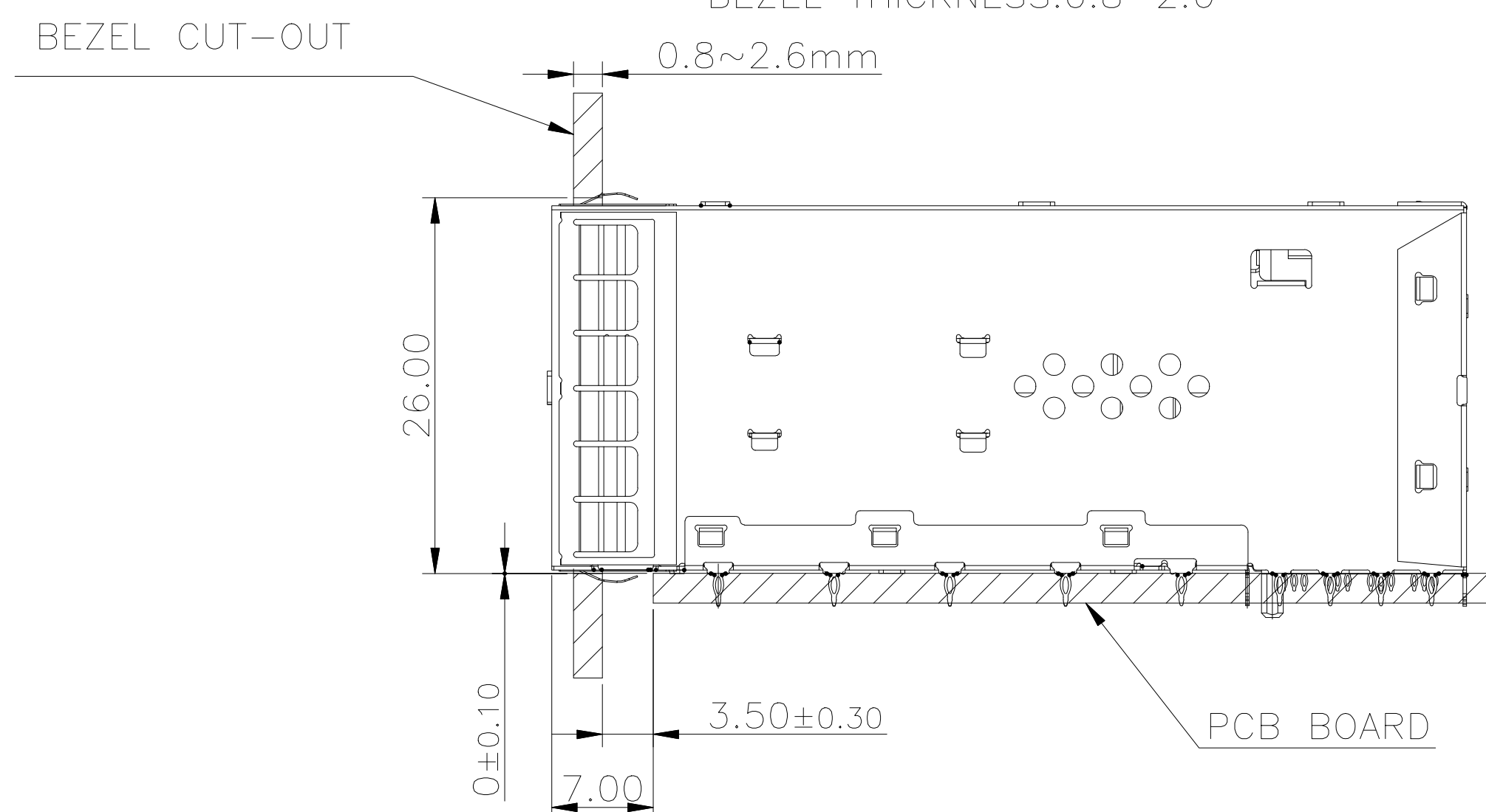
BEZEL CUT-OUT CENTER SPACING DETAIL BEZEL THICKNESS:0.8-2.6
