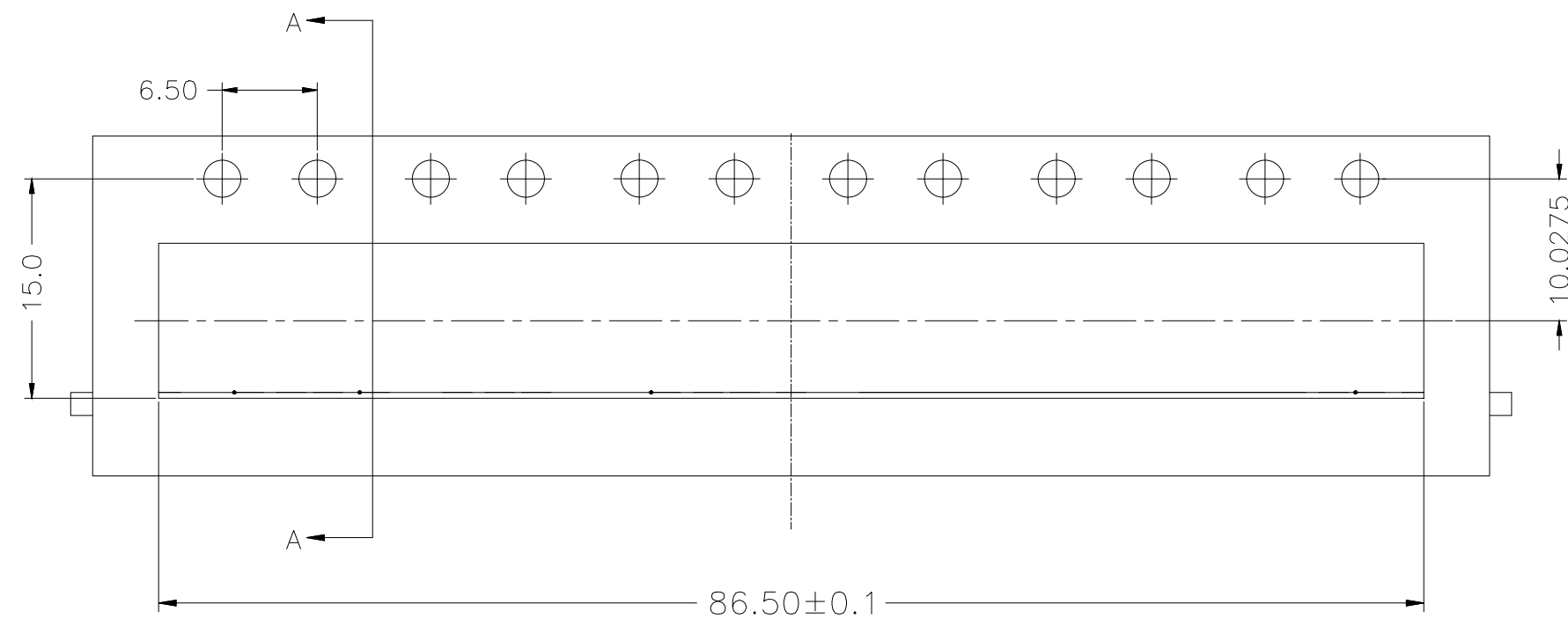
MOUNTED ON PC BOARD SHOWN THRU RECOMMENDED BEZEL
