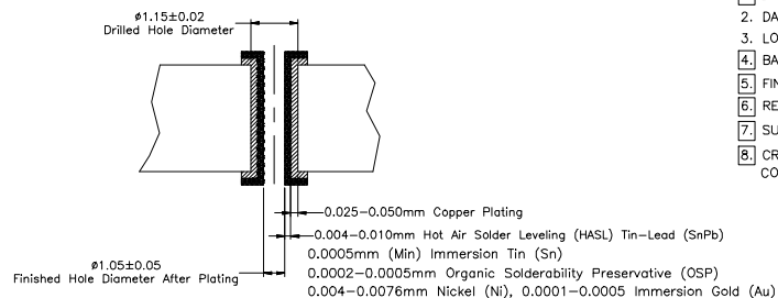
FINISHED HOLE SIZE SPECS
