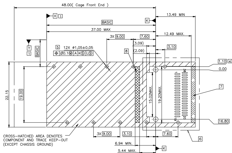
RECOMMENDED SINGLE SIDE PC BOARD LAYOUT
