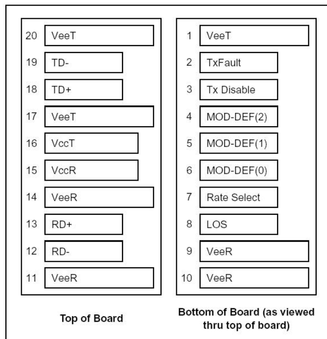
Figure 1:Pin Diagram
