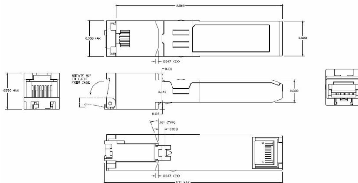
Figure 2. mechanical dimensions
