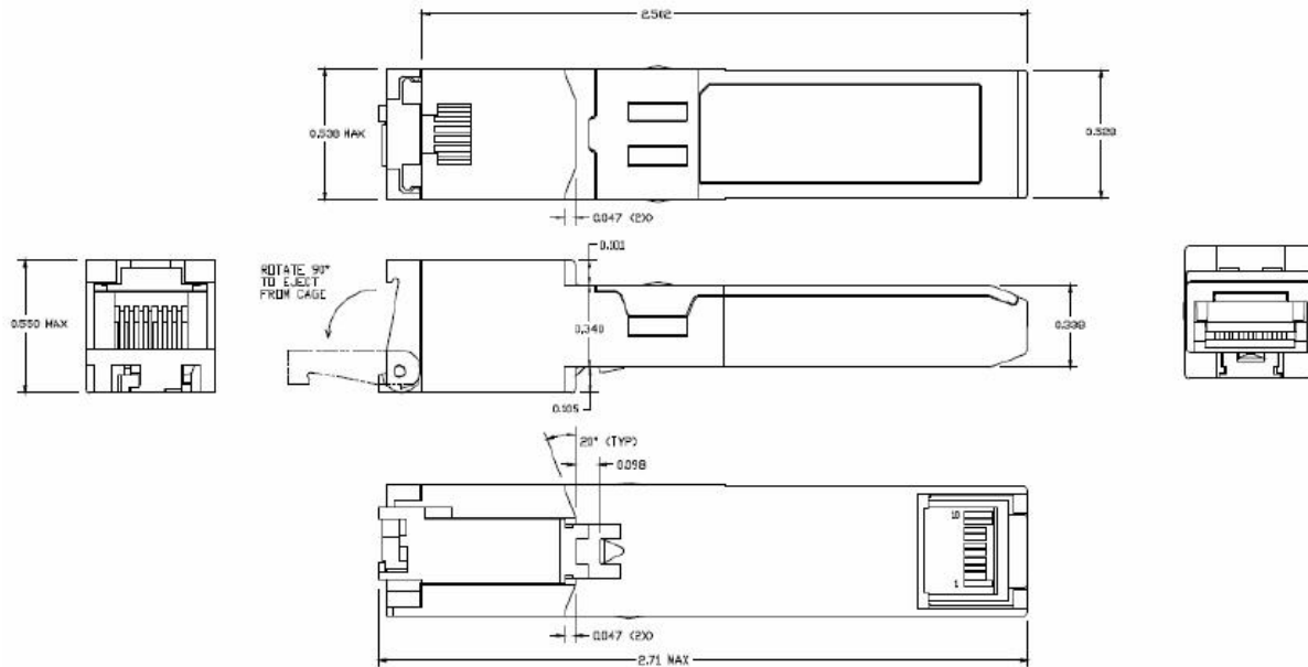
Figure 2. mechanical dimensions
