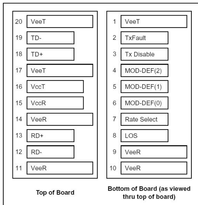
Figure 1:Pin Diagram
