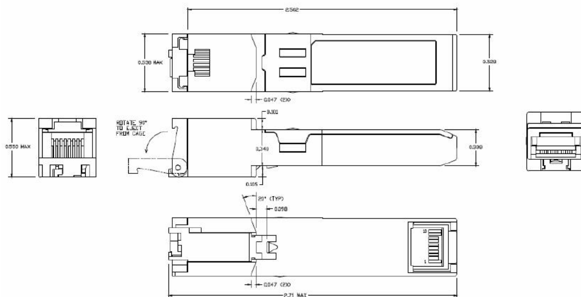
Figure 2. mechanical dimensions
