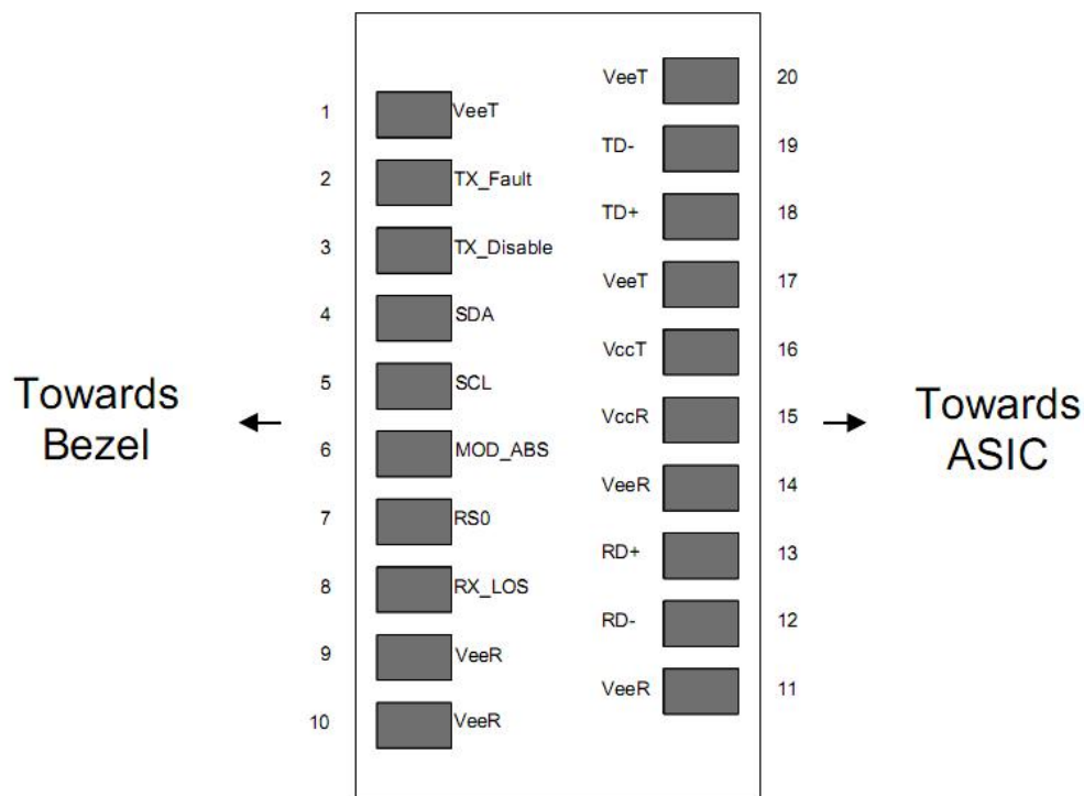
Figure 1:Pin Diagram
