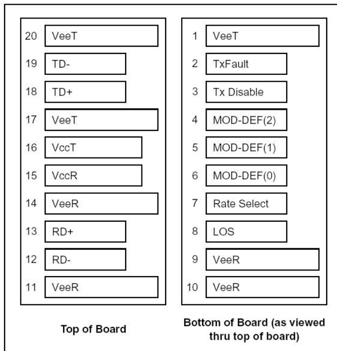
Pin Diagram
