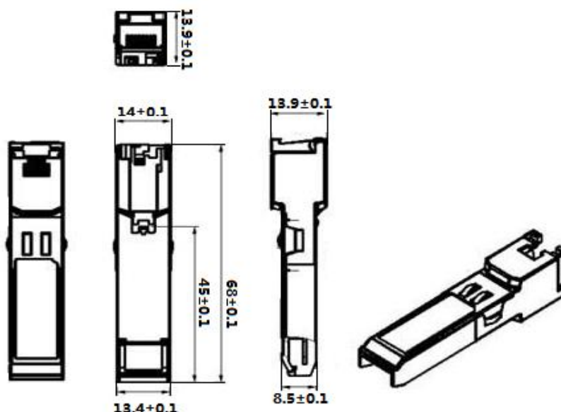
Figure 2. Mechanical dimensions
