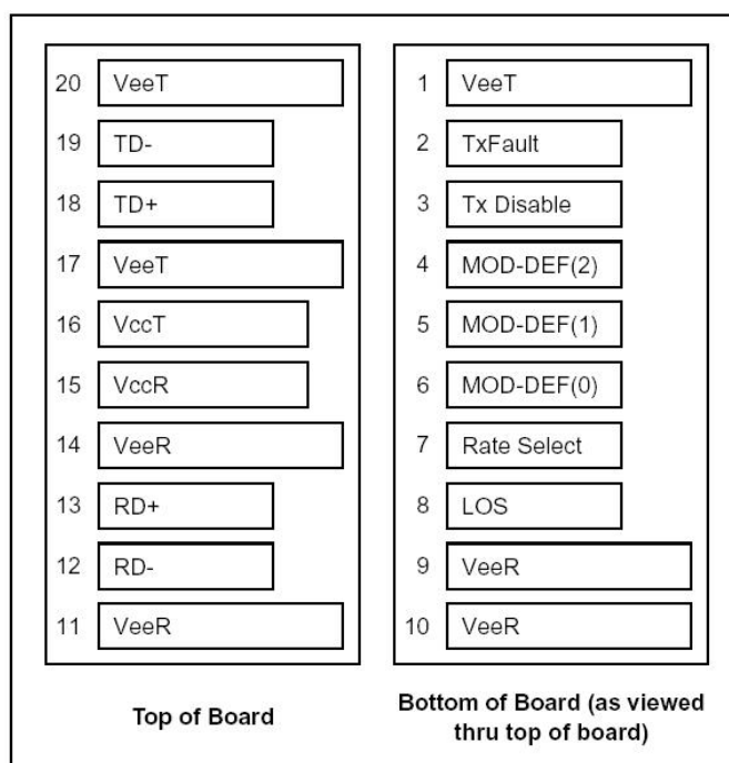
Figure 1:Pin Diagram
