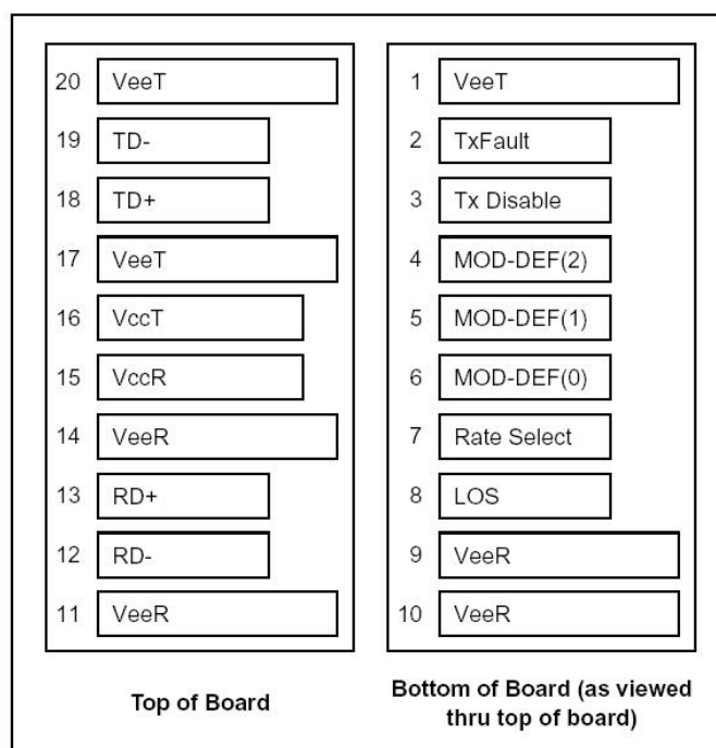
Figure 1:Pin Diagram
