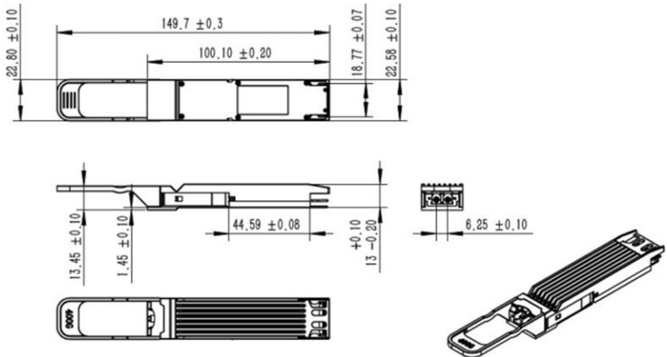
Mechanical Dimensions
