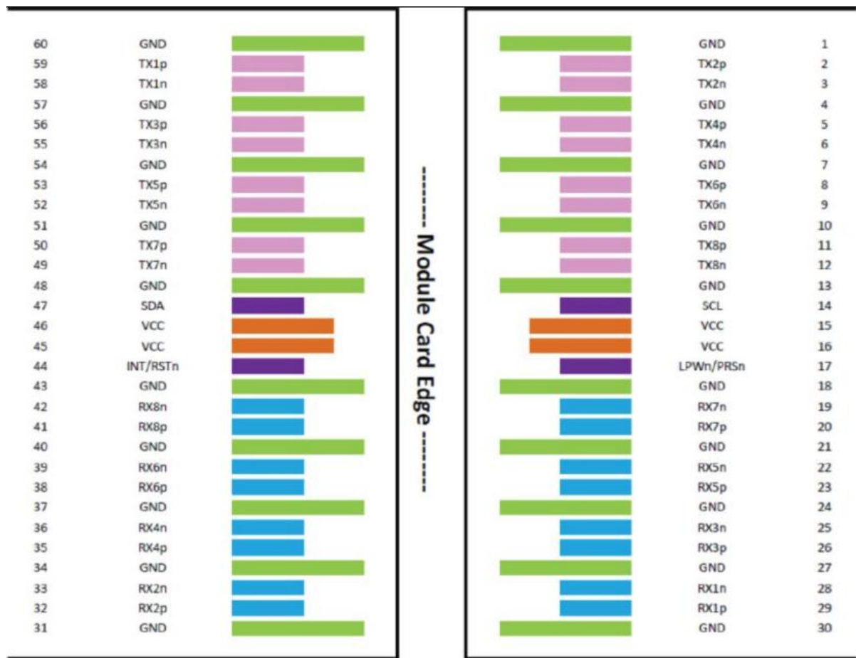
Figure 1. MSA Compliant Connector
