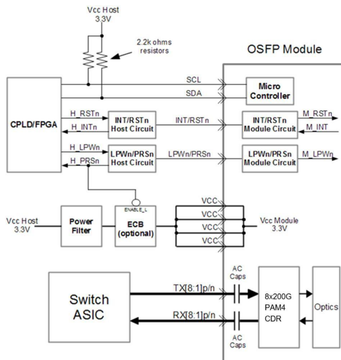
Figure 2 – Recommended OSFP Host Board Schematic
