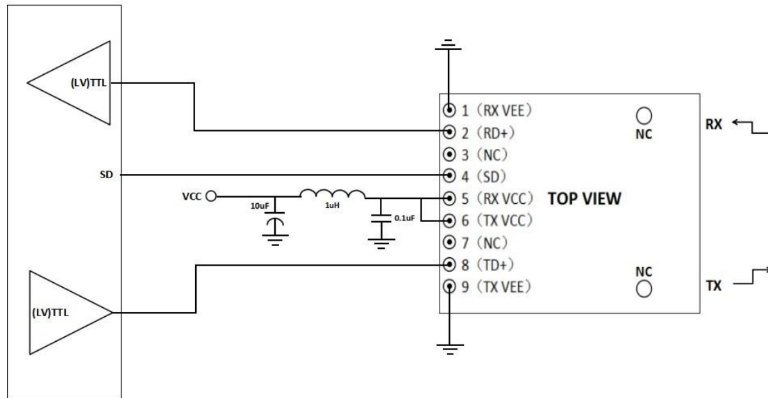
Recommended Circuit Schematic
