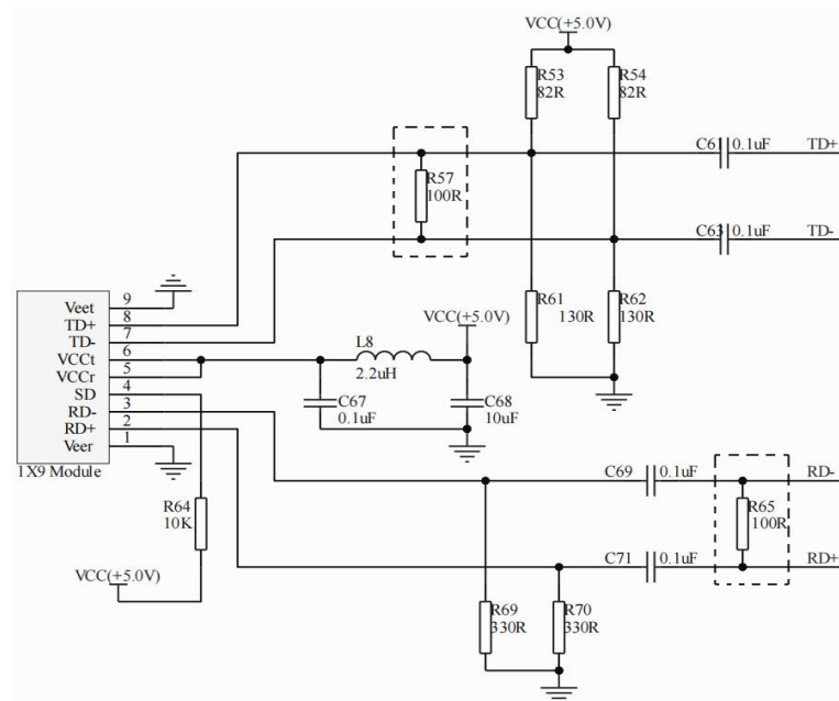
Recommended Circuit Schematic 5V SD TTL
